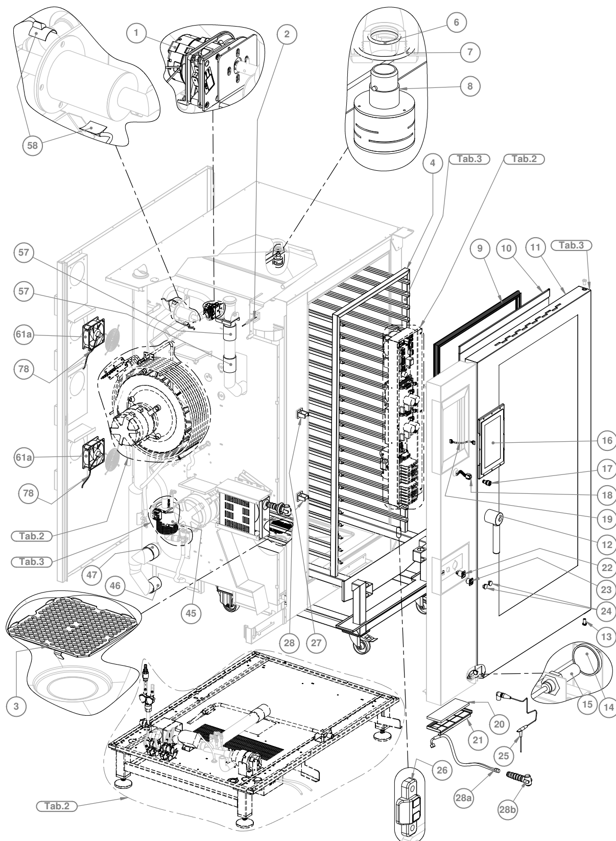
Exploded view 1/3
