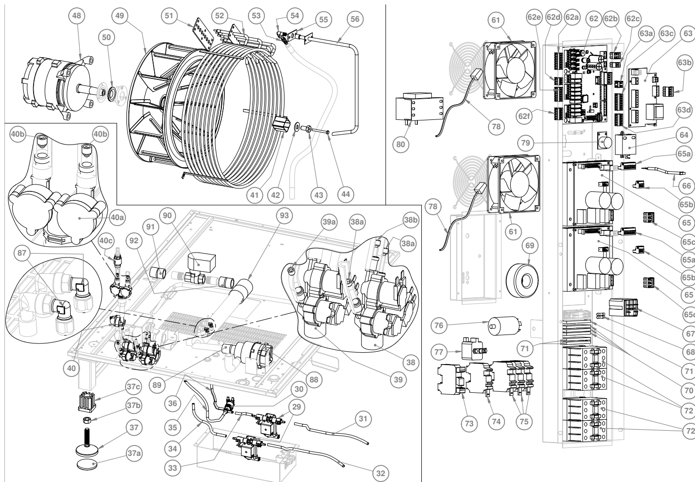
Exploded view 2/3
