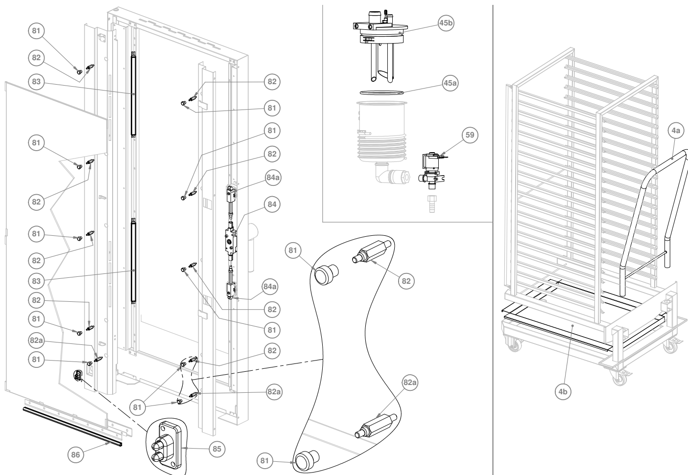
Exploded view 3/3
